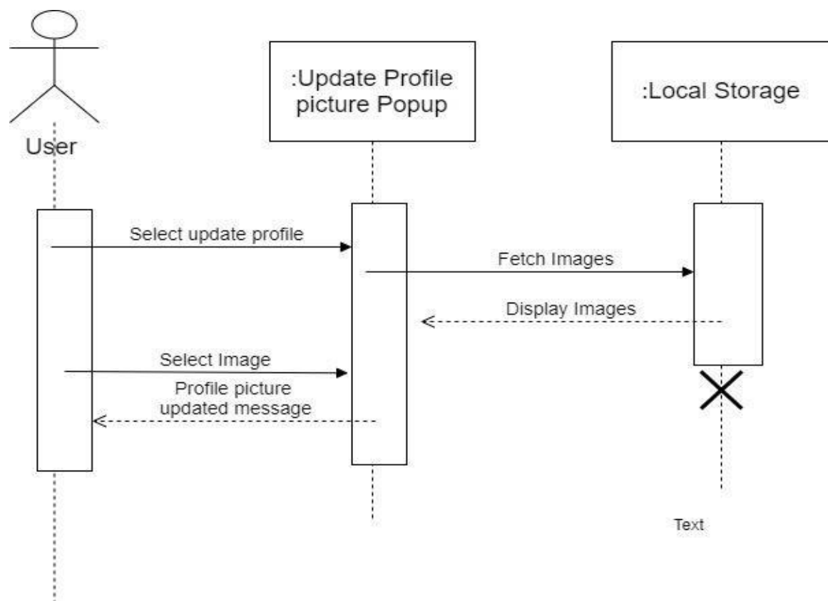
Fig 5.3(E) Sequence Diagram for changing profile
